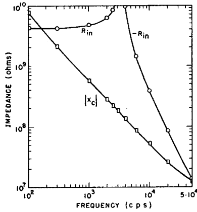
FIG. 2. Frequency variation of resistance and capacitive reactance to ground at coaxial cable input of high input impedance circuit.
